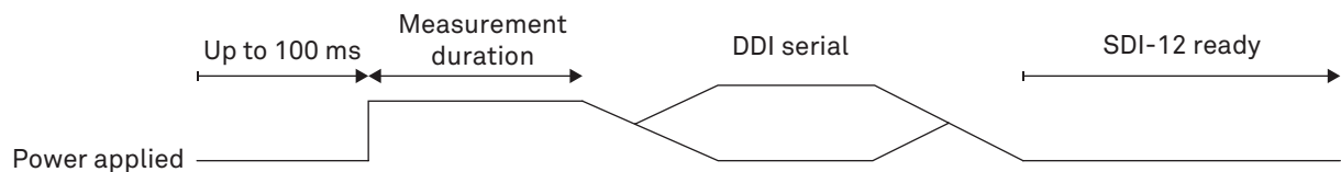
Figure 9 Data line DDI serial timing
